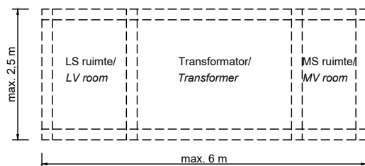
Plattegrond transformatorstation/ Ground plan transformer station
