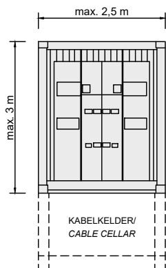
Zijaanzicht transformatorstation/ Side view transformer station
